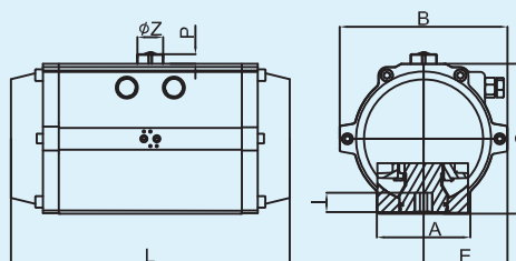
VT New Series Pneumatic Actuator Dimension Table (Unit: mm)
